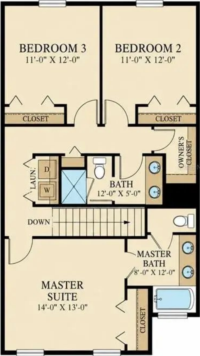
SECOND FLOOR
